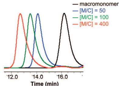
Figure 3. GPC traces of macromonomer NB(PtBA)4700 (black) and crude brush polymers PNB-g-PtBA obtained at [M/C] = 50 (blue), 100 (green), and 400 (red). Conditions: [M]_0 = 0.05 M in THF at room temperature.
