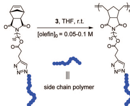
Scheme 4. Synthesis of Polymacromonomer from \omega -Norbornenyl MM
