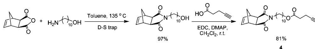
Scheme 2. Synthesis of Monomer 4
