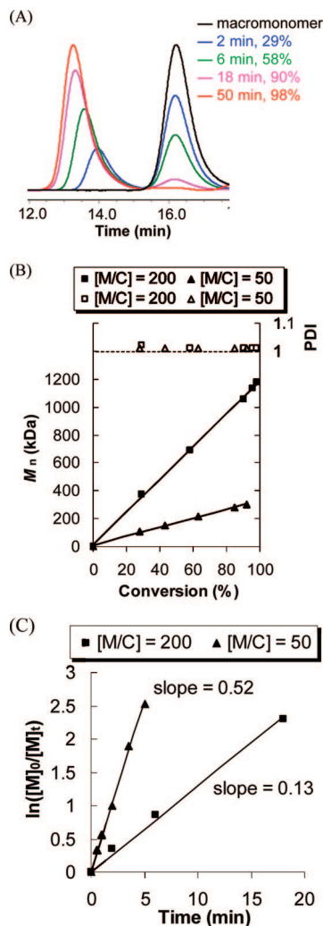
Figure 2. (A) Evolution of GPC traces during ROMP of NB(PtBA)4700; (B) dependence of M_n and PDI on MM conversion; and (C) dependence of \ln([M]_0/[M]_t) on time. Conditions: [M]_0 = 0.05 M in THF at room temperature.
