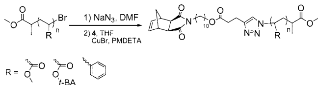
Scheme 3. Synthesis of Macromonomers
