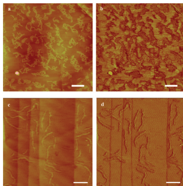
Figure 4. Tapping-mode AFM images of brush polymer PNB-g-PS (entry 14 in Table 2) spin-cast from chloroform solution onto HOPG. (a,b) Large-scale height and phase images, bar = 300 nm; (c,d) enlarged height and phase images, bar = 100 nm.
